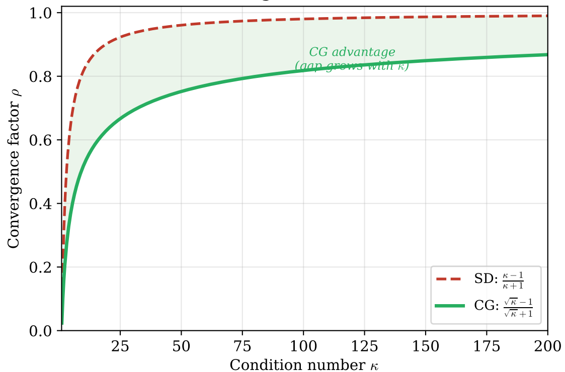
Convergence factor vs. \kappa
